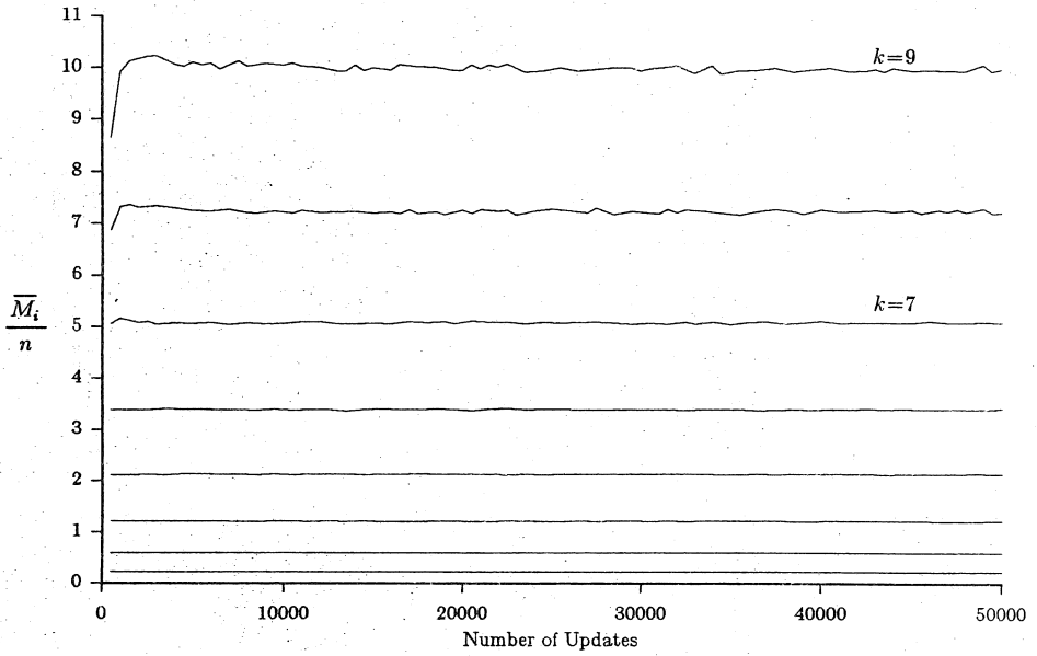
Figure 4a. Simulation results for n=2^k-1 , k=2..9 .
