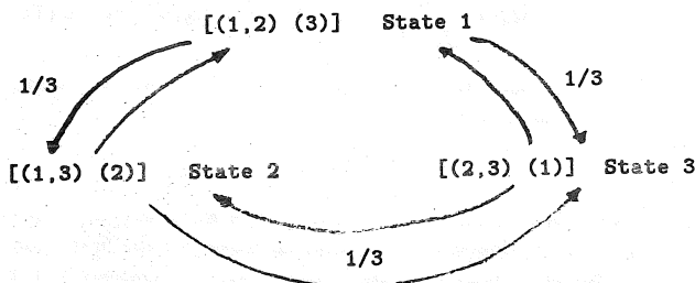
Figure 3: Markov chain for n = 3 .
