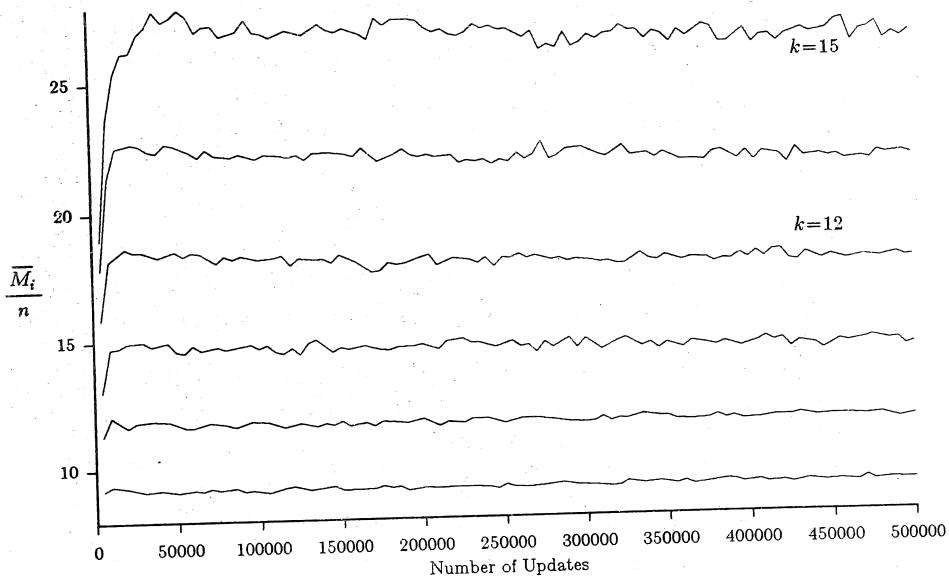
Figure 8b. Simulation results (new algorithm) for n=2^k-1 , k=10..15
