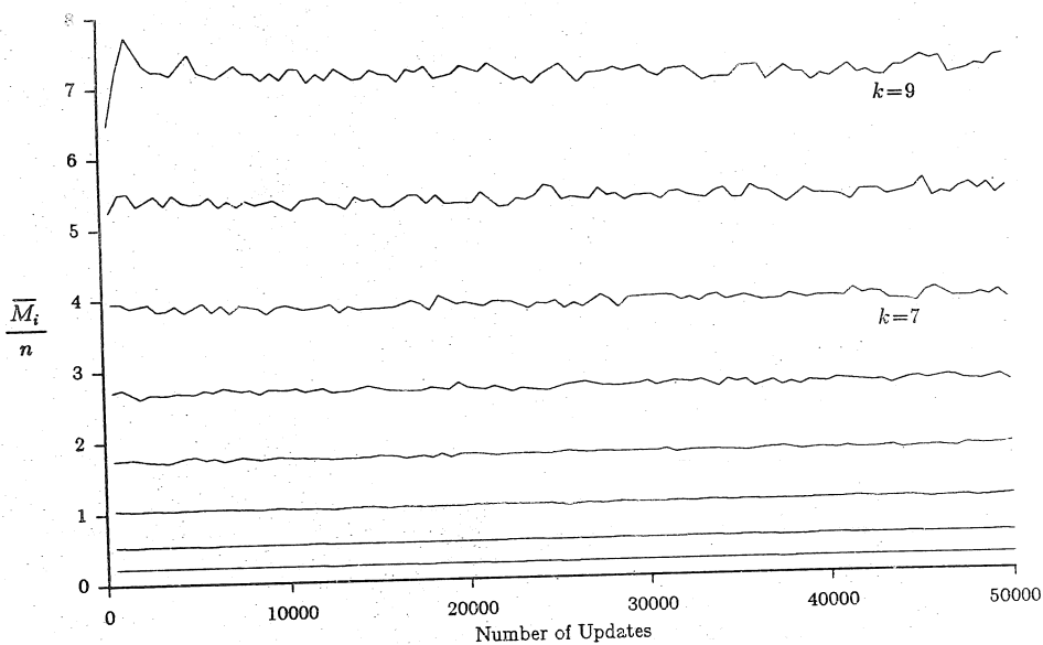
Figure 8a. Simulation results (new algorithm) for n=2^k-1 , k=2..9
